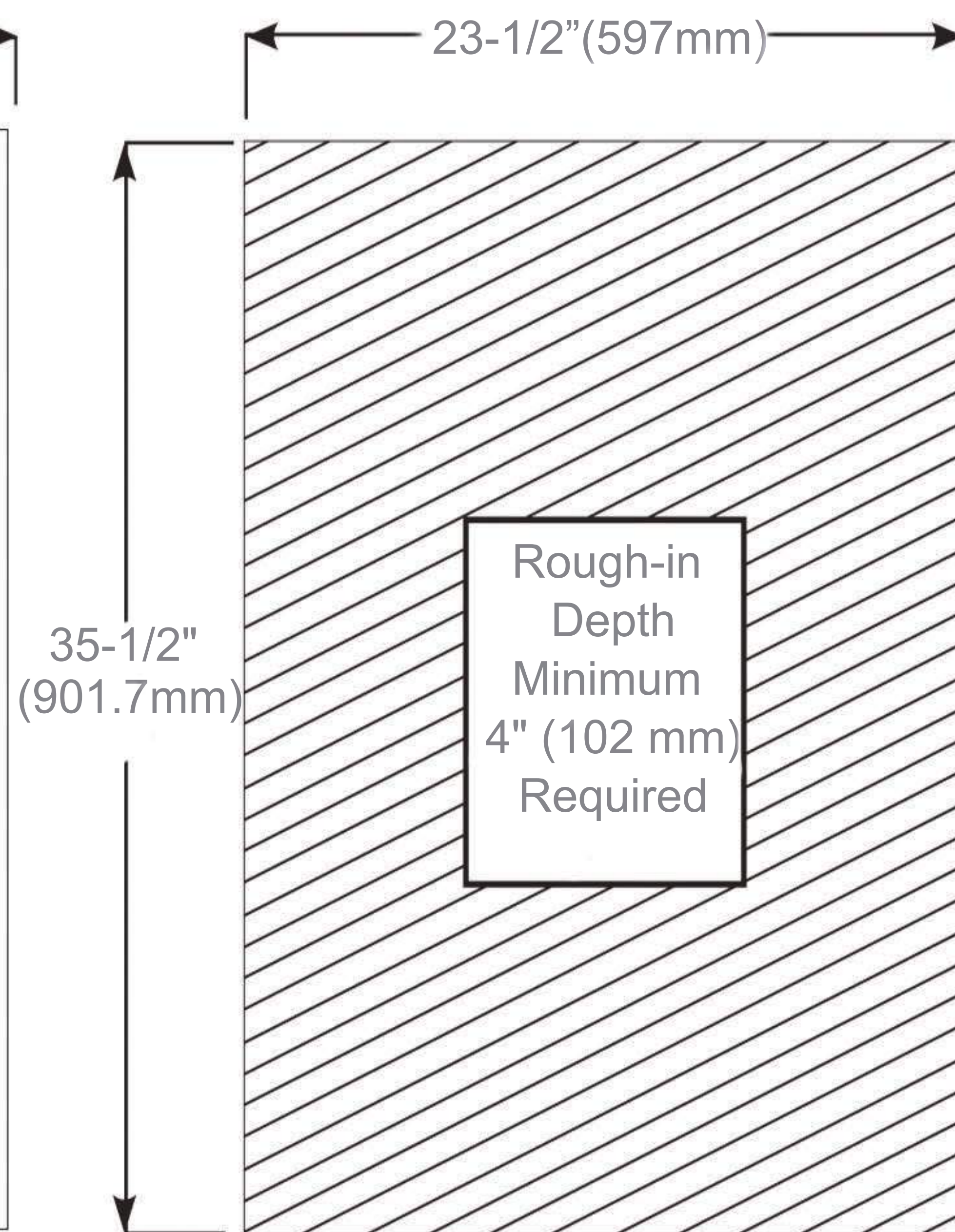
Rough-in Dimensions
