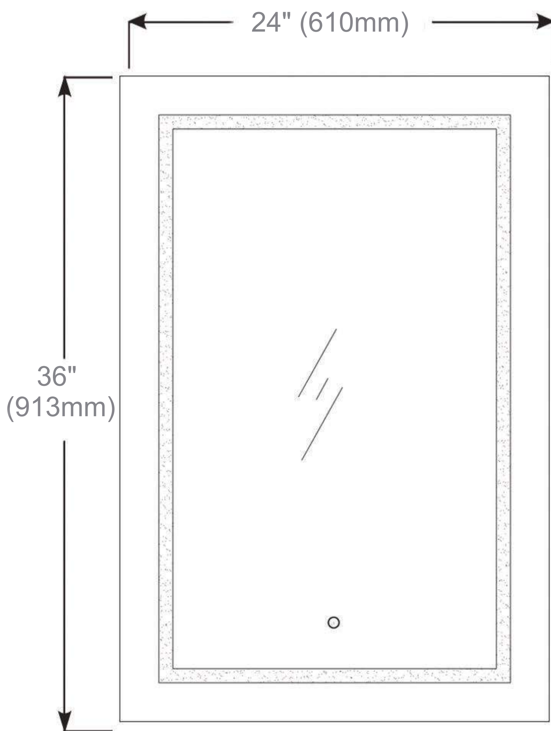
Cabinet Dimensions
