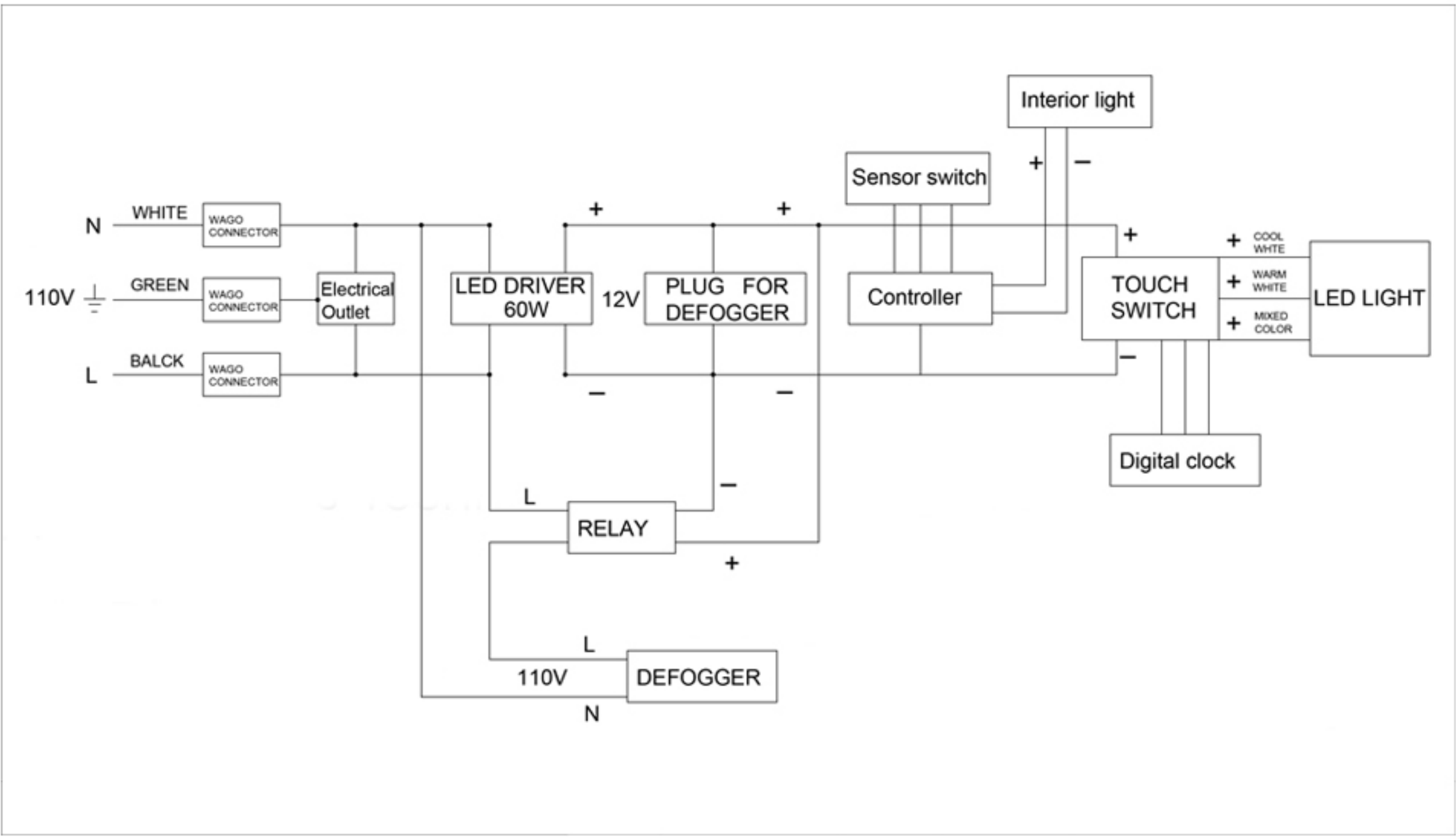
Circuit Diagram
