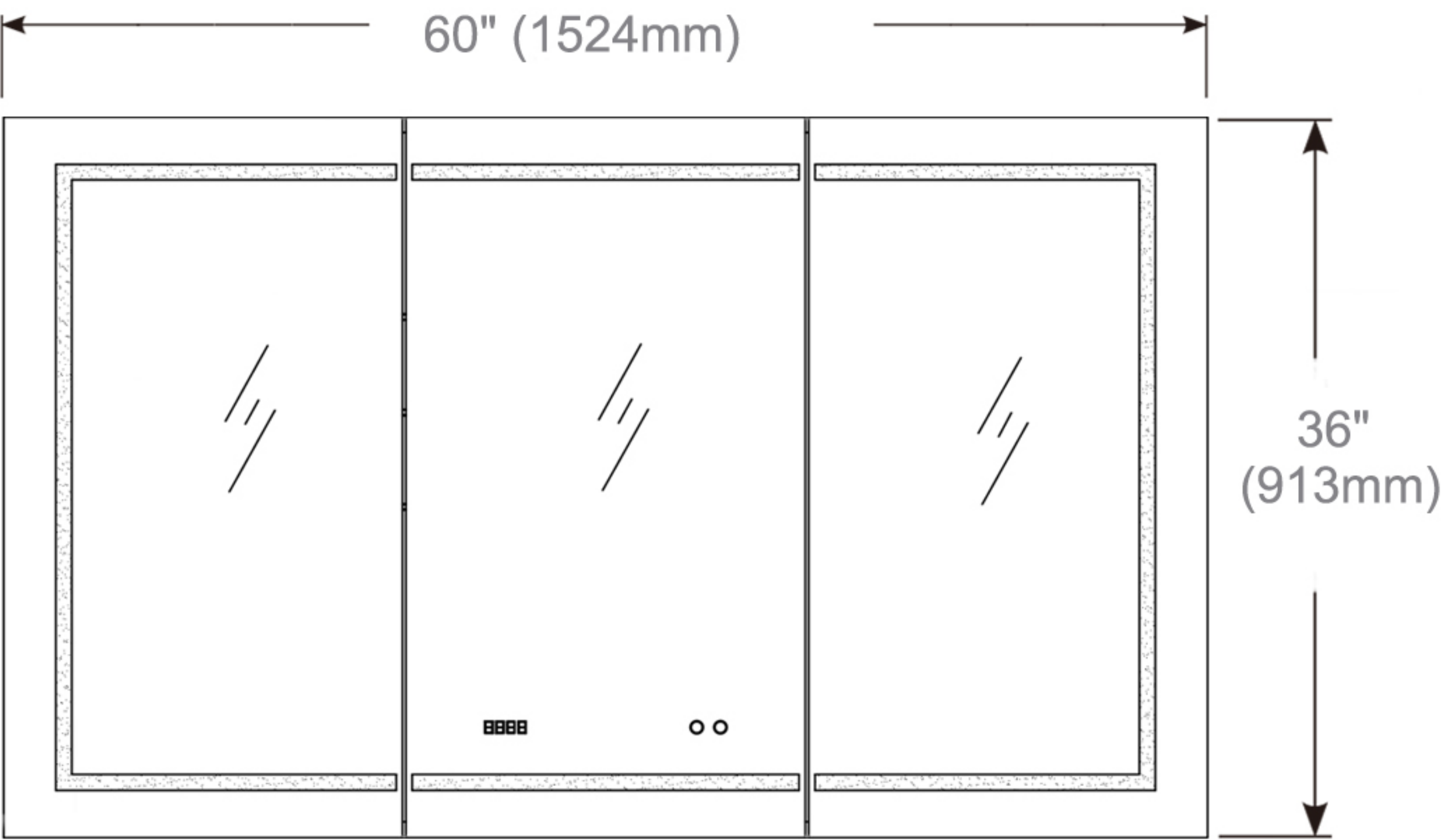
Cabinet Dimensions
