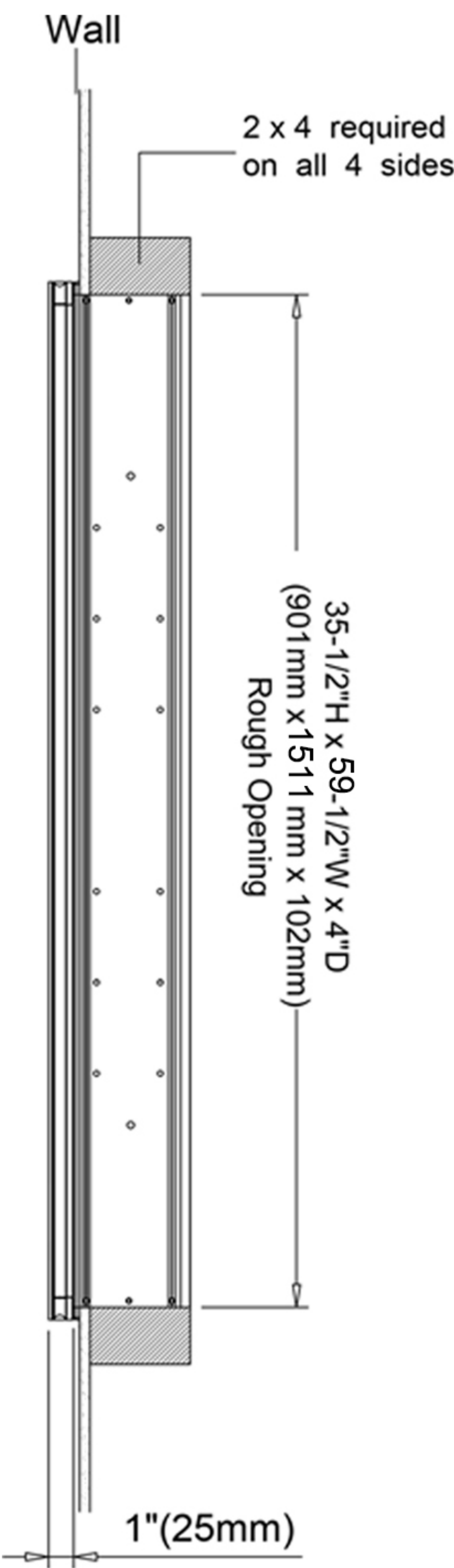
Recessed Mount
