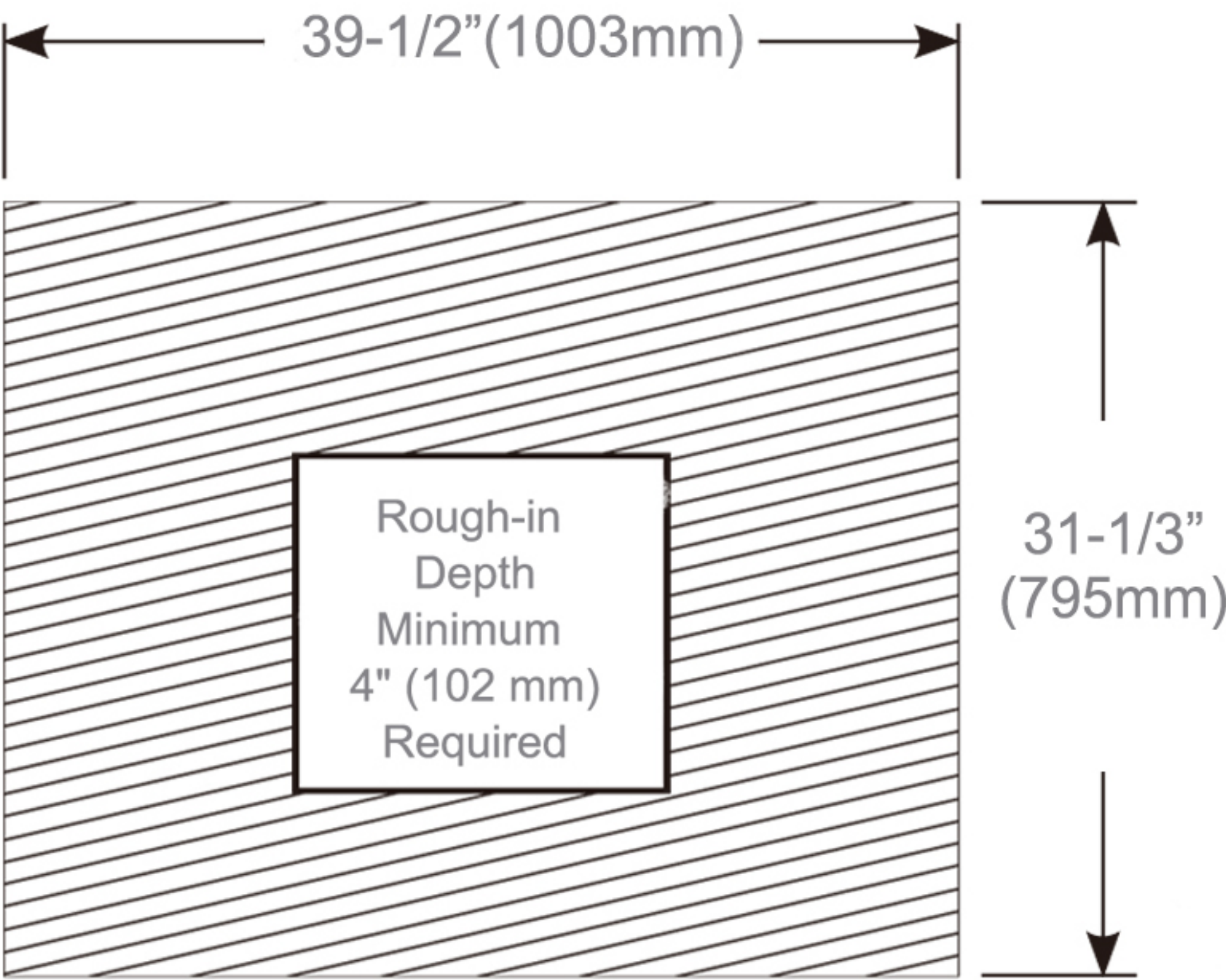
Rough-in Dimensions
