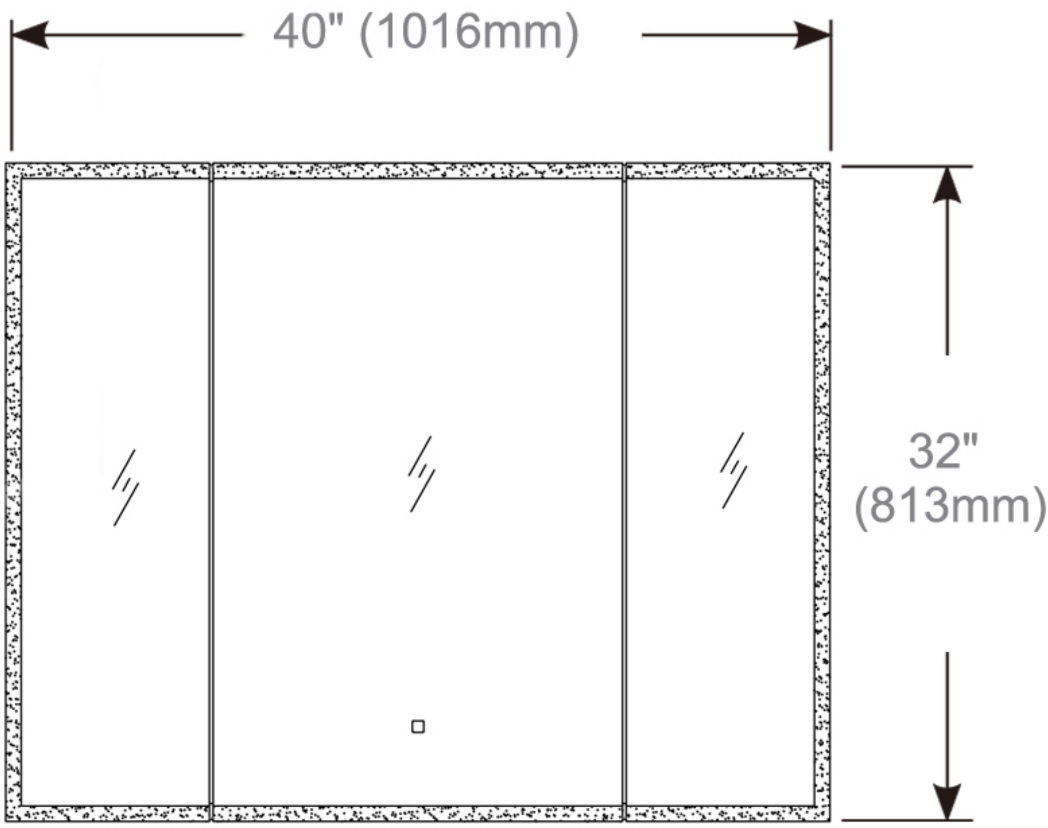
Cabinet Dimensions
