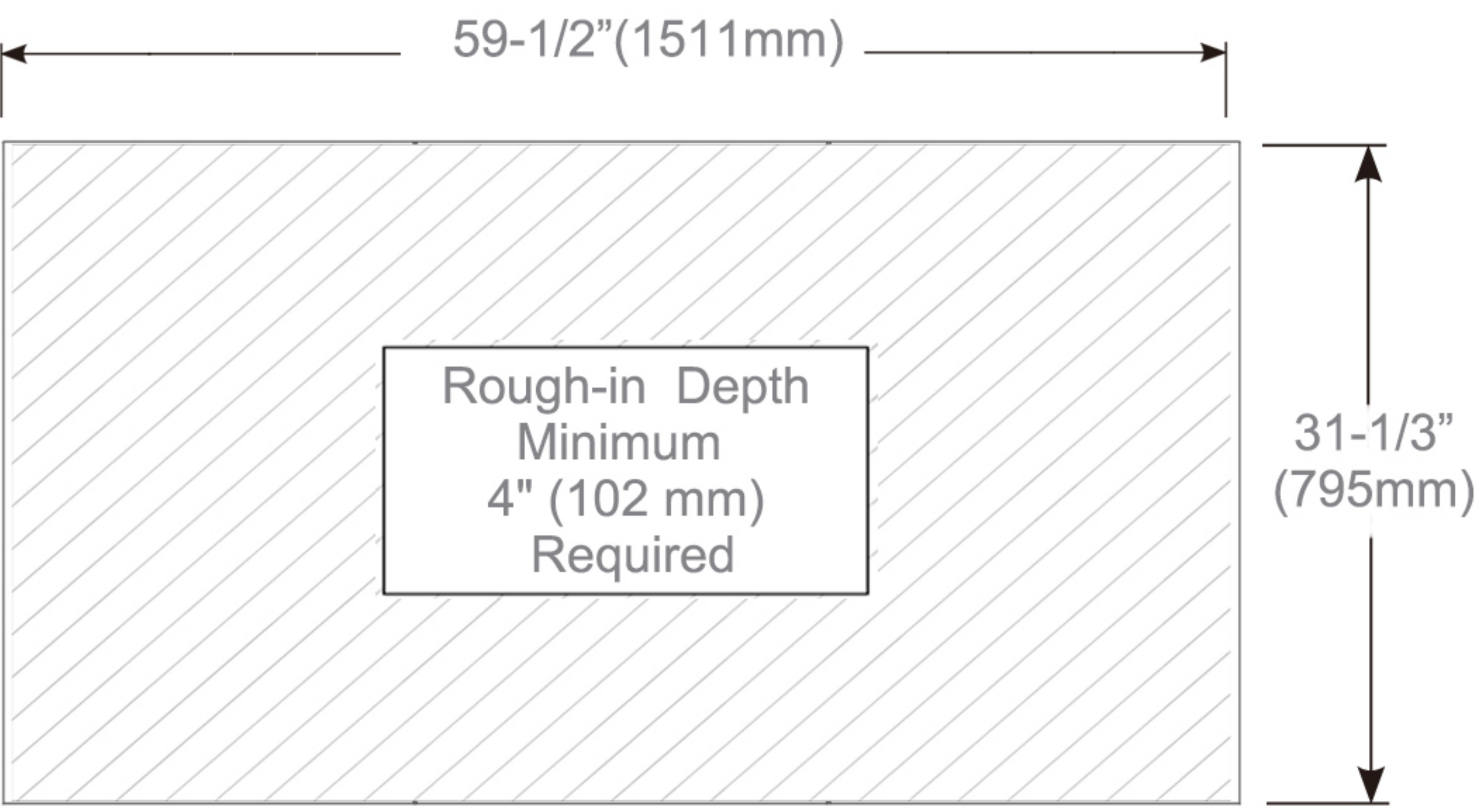
Rough-in Dimensions
