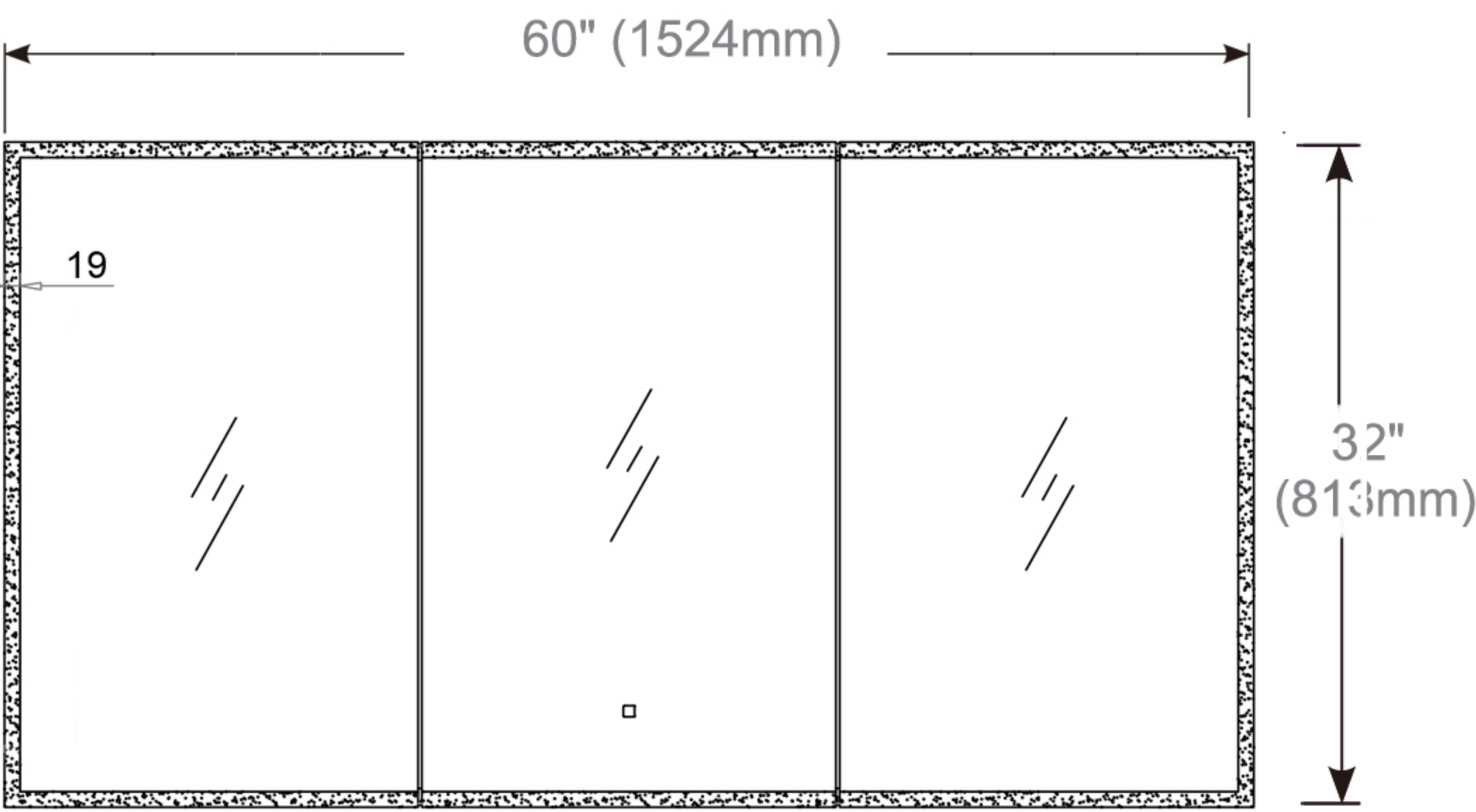
Cabinet Dimensions
