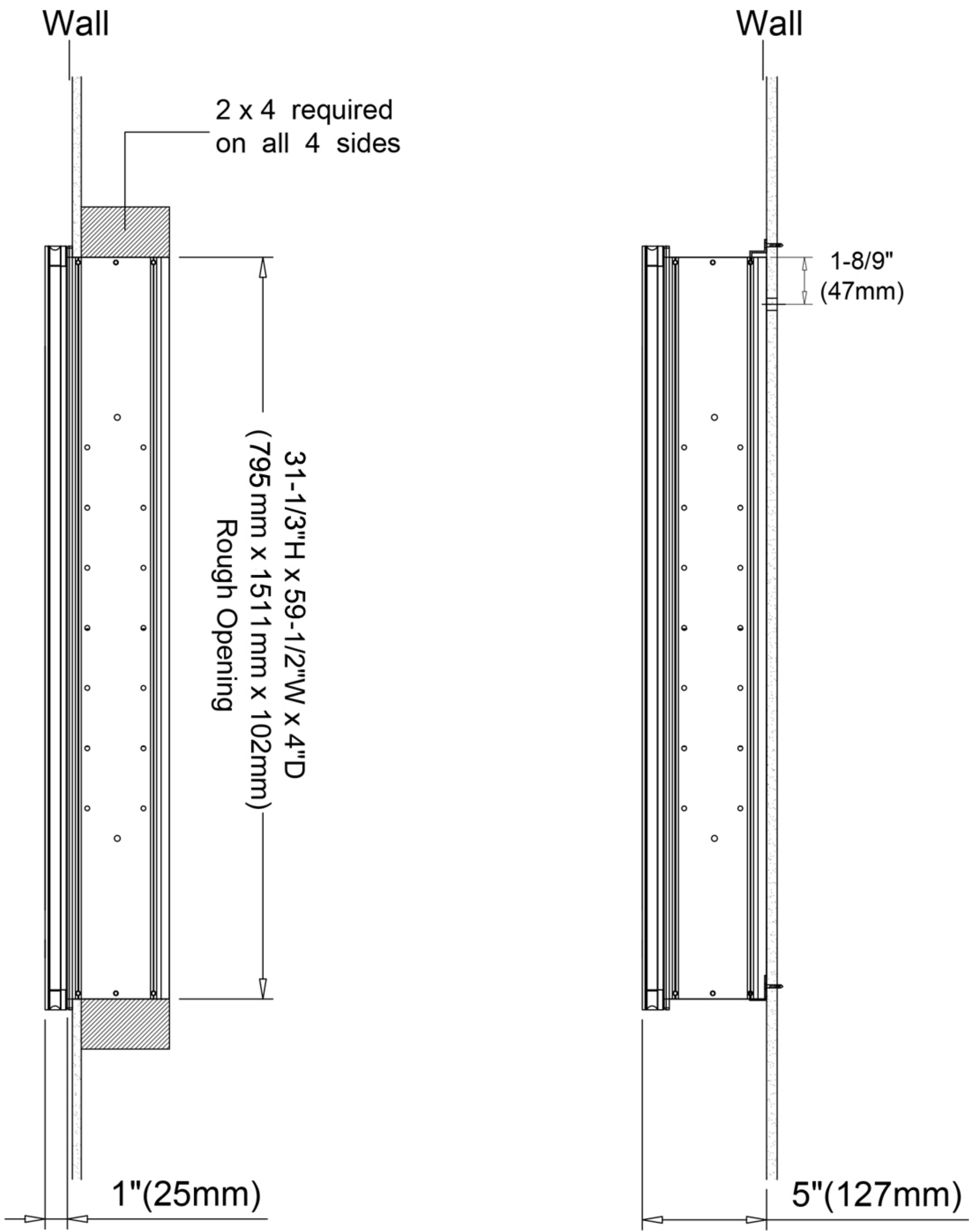
Recessed Mount
