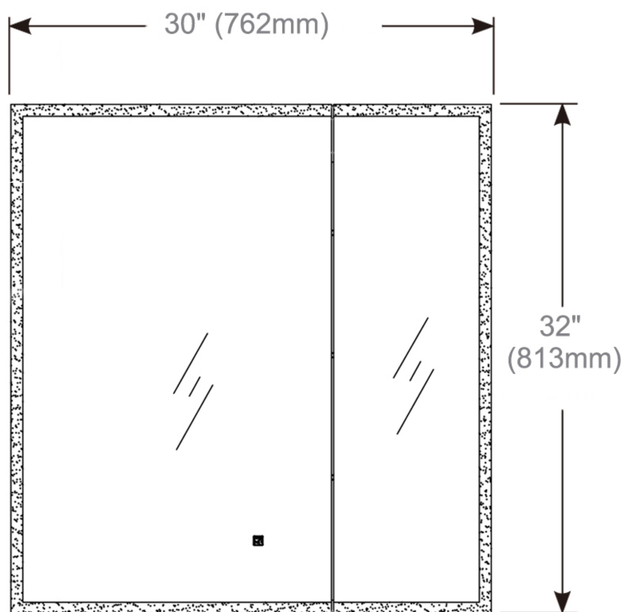
Cabinet Dimensions
