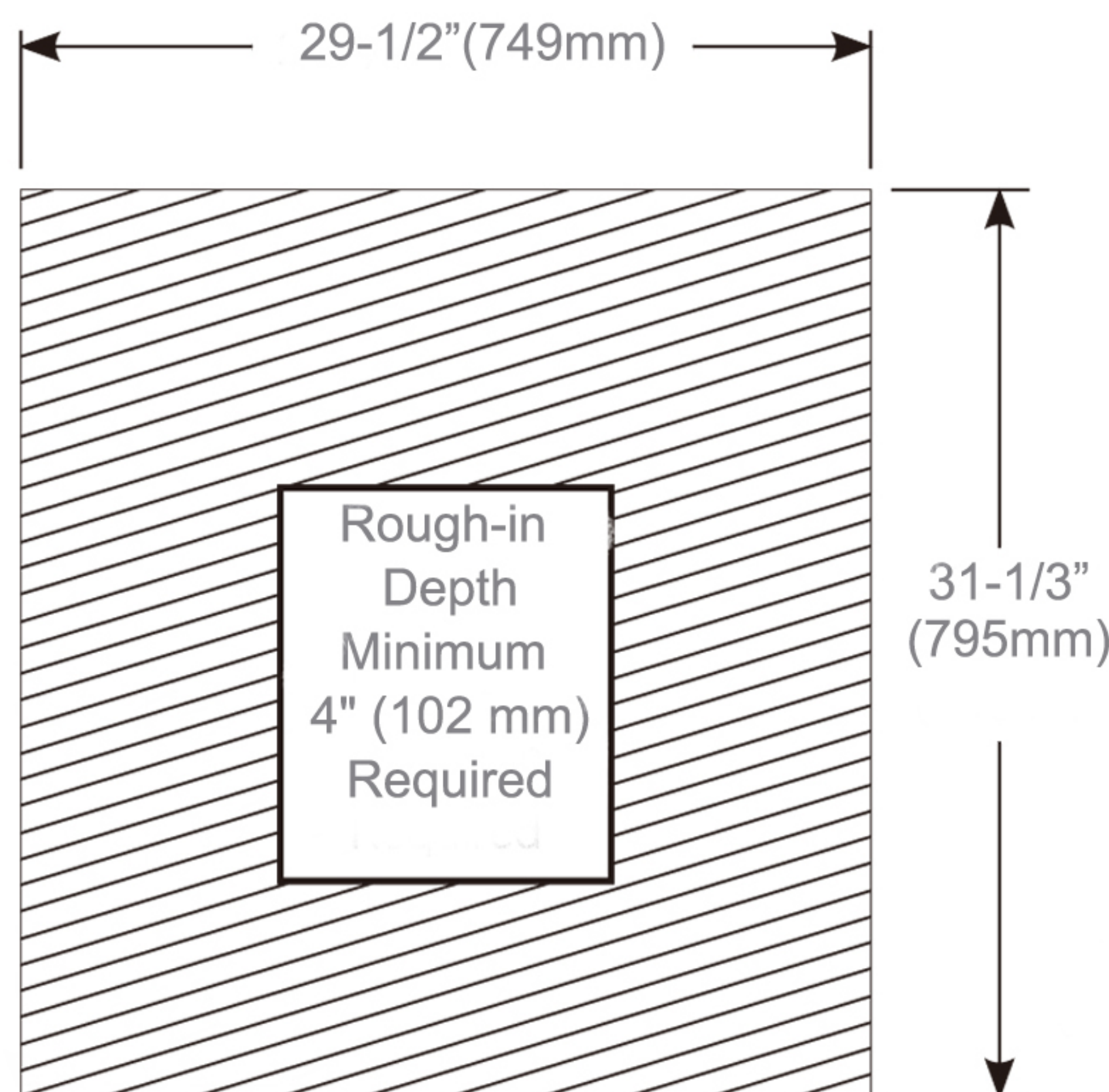
Rough-in Dimensions
