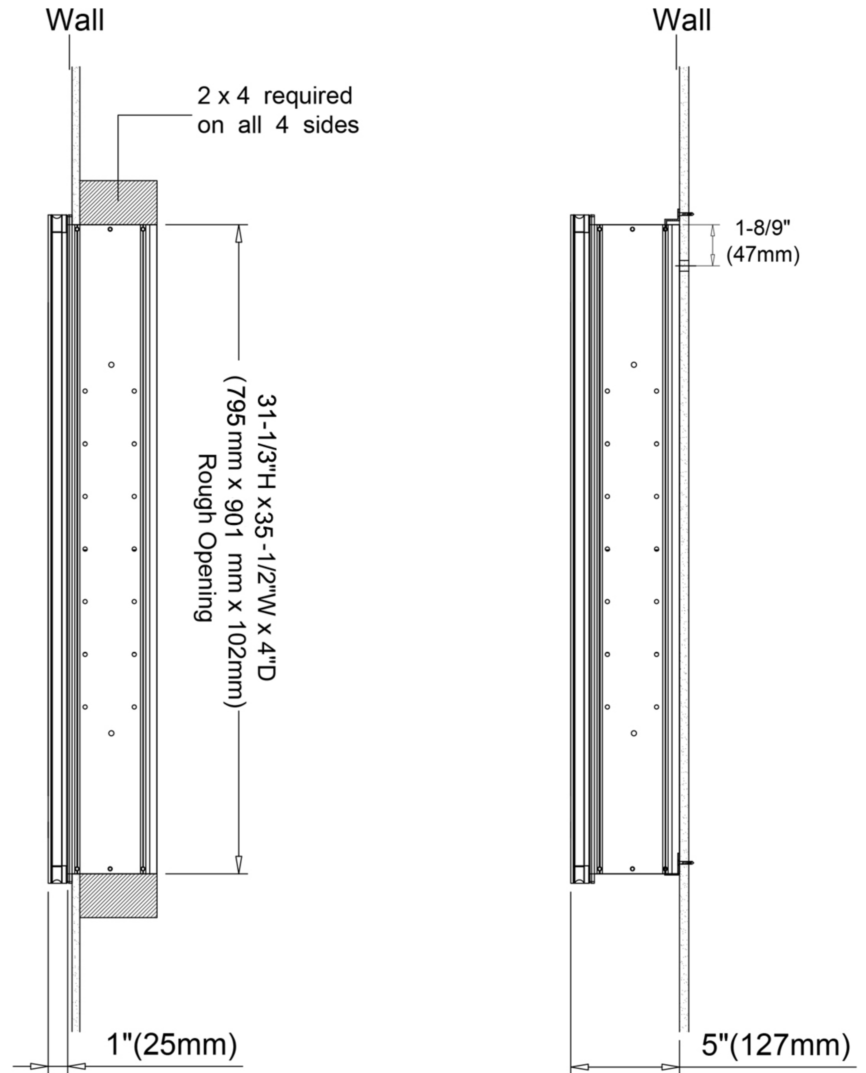
Recessed Mount
