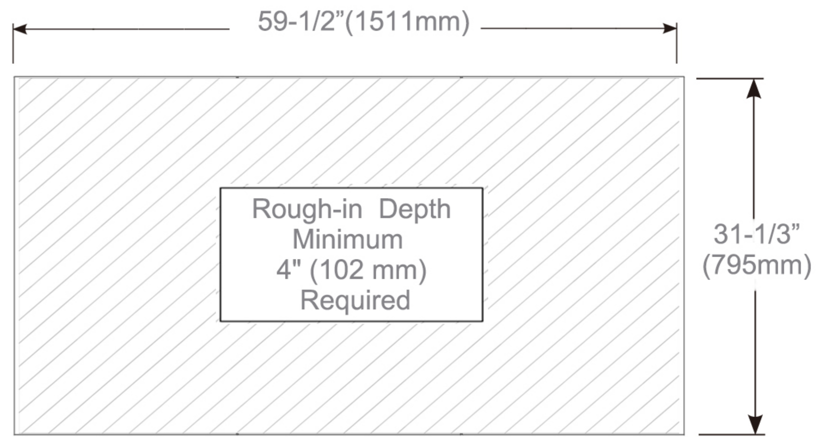
Rough-in Dimensions
