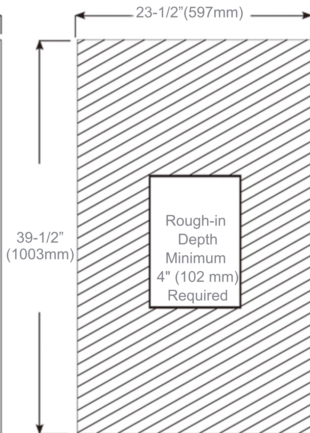
Rough-in Dimensions
