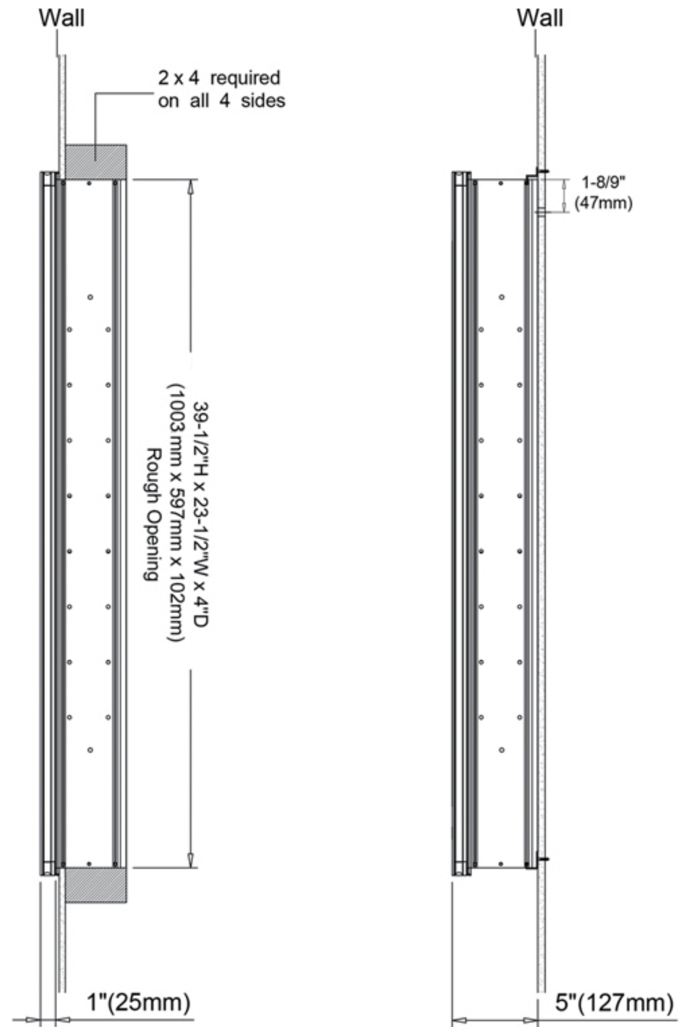
Recessed Mount
