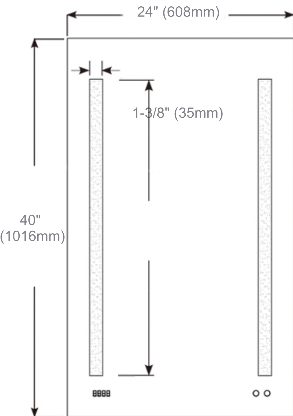
Cabinet Dimensions
