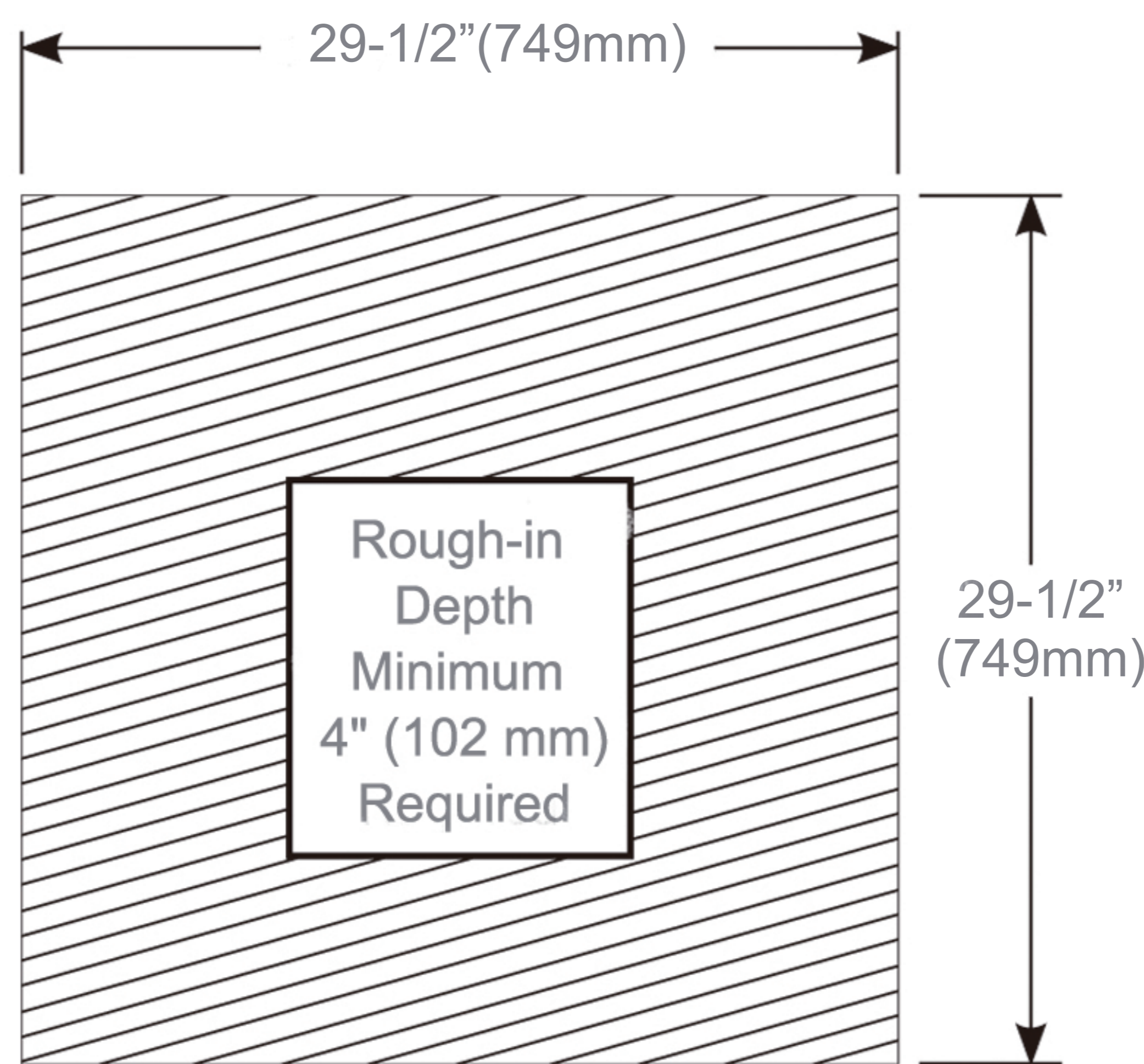
Rough-in Dimensions
