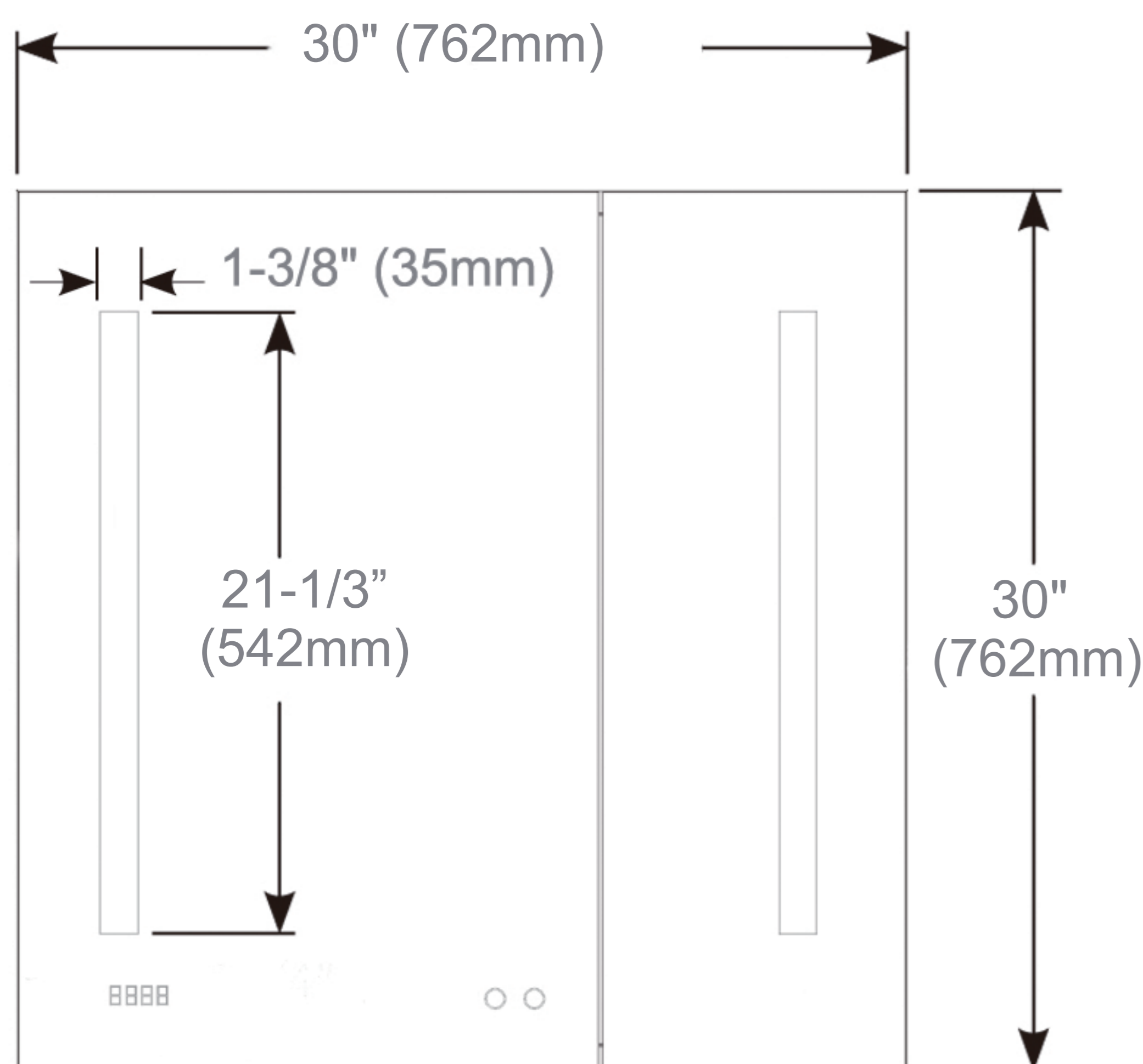
Cabinet Dimensions
