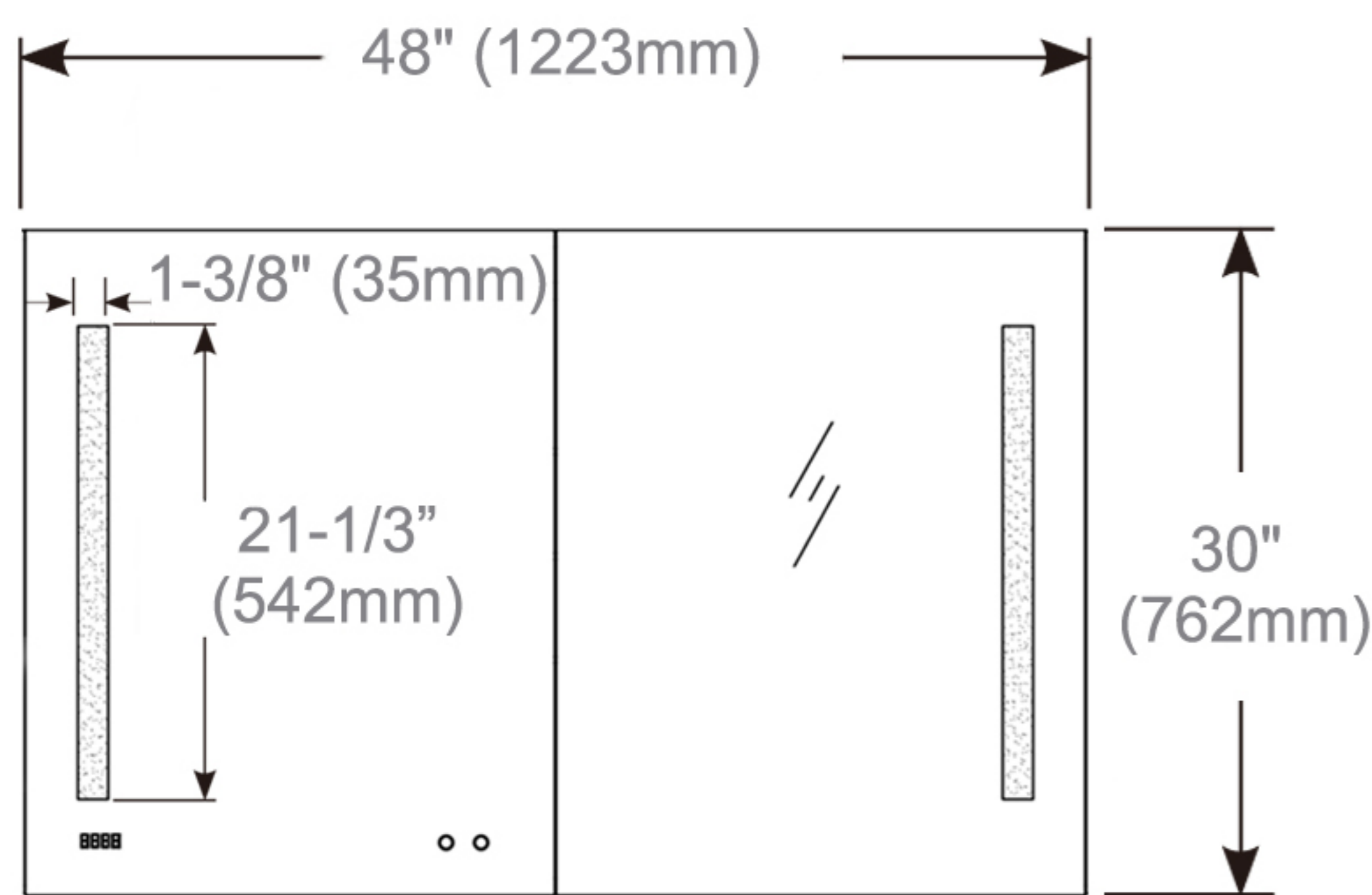
Cabinet Dimensions
