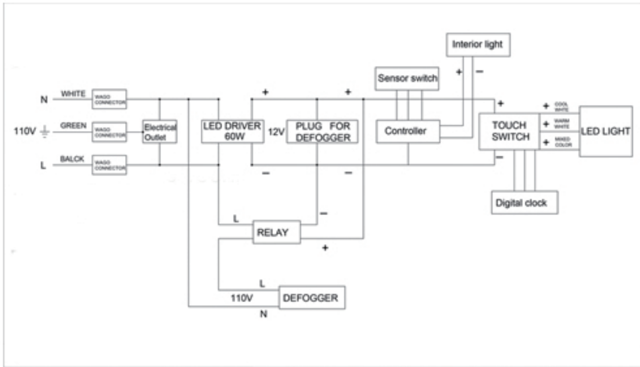
Circuit Diagram
