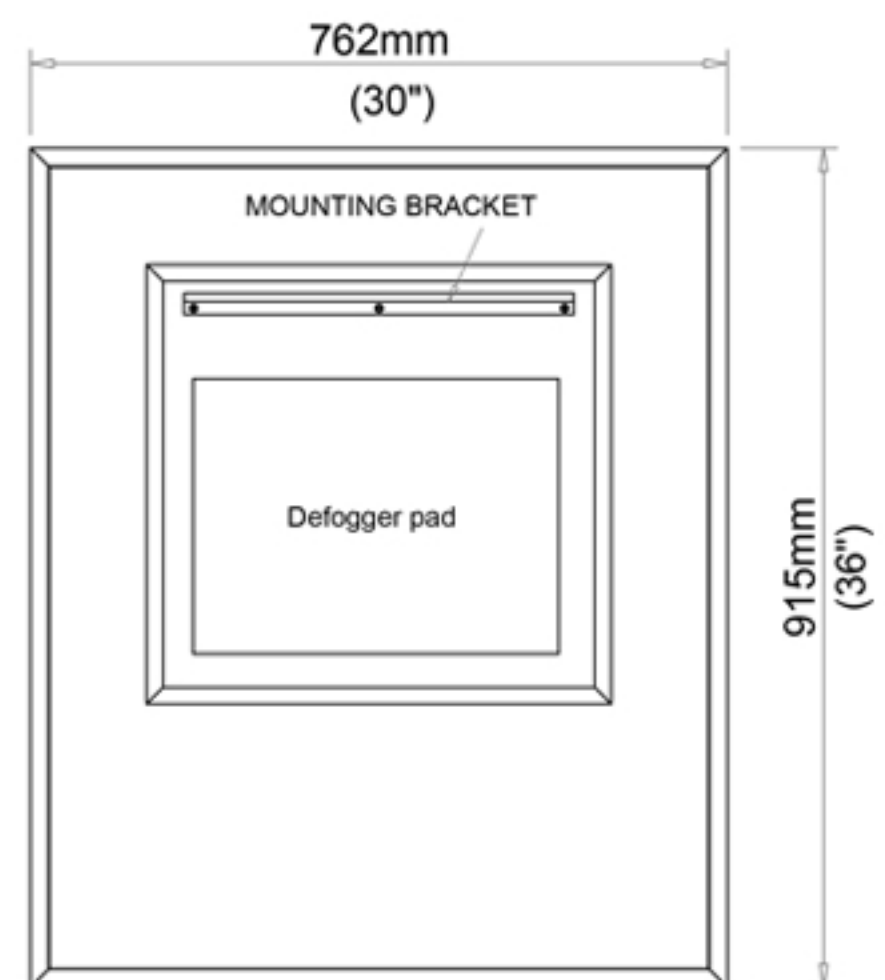
Back view for electrical knockout location
