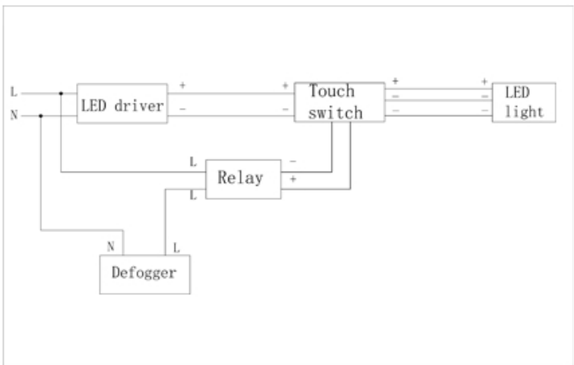
Circuit diagram
