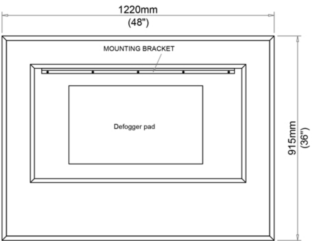
Back view for electrical knockout location
